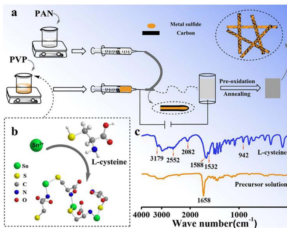
Fig. 14 (a) Pictorial representation of synthesis procedure of SnS@CF via electrospinning, (b) structure of the chelate complex formed by L-cysteine and metal cation, and (c) FTIR spectra of L-cysteine and mixed solution of SnCl 2 and L-cysteine. Reproduced with permission from ref. 39. Copyright (2019), American Chemical Society.
