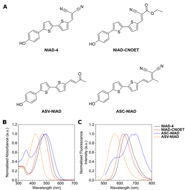
Fig. 1 (A) Chemical structures of NIAD-4 and derivatives used in this study. Comparison of (B) normalized absorbance and (C) emission spectra of all dyes measured in DMSO. Excitation wavelength of 488 nm used for NIAD-4, NIAD-CNOET, and ASC-NIAD and 405 nm used for ASV-NIAD. Dye concentration was 10 \mu M for all measurements.
