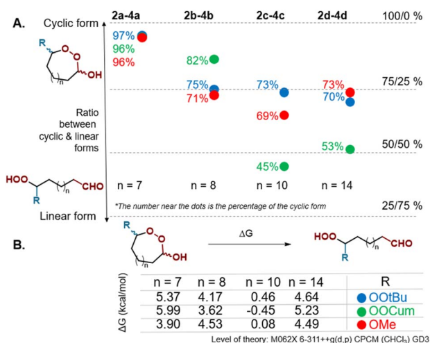
Scheme 6 Ratio of cyclic and linear forms of compounds 2a–d , 3a–d , and 4a–d after column chromatography (by ^1\text{H} NMR, A) and \Delta\text{G} of the cycle opening (by DFT, B).
