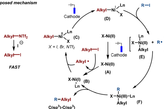
Scheme 24 Proposed mechanism.
