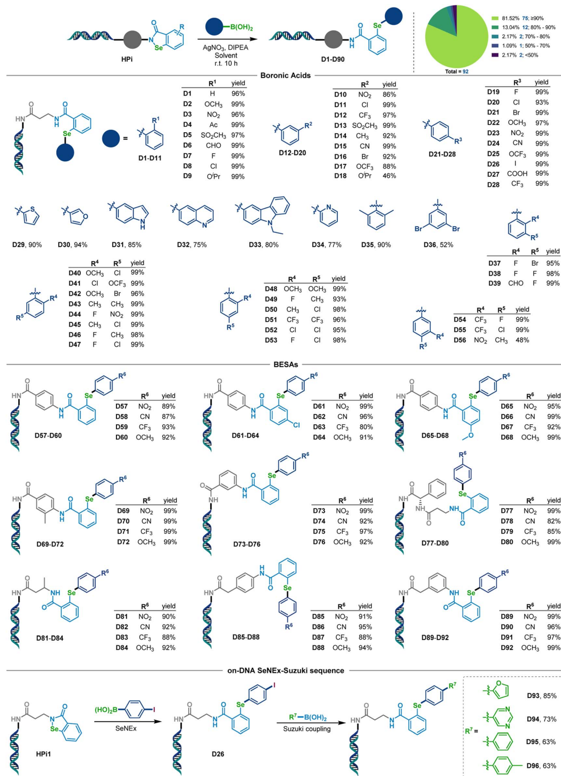
Fig. 7 Scope of the on-DNA SeNEx reaction of DNA-conjugated BSEAs and boronic acids. Standard reaction conditions: 1 equiv. of HPI (1 mM in ddH 2 O), 10 equiv. of AgNO 3 (10 mM in ACN), 1000 equivalents of DIPEA (1 M in ACN), 1000 equiv. of boronic acid (1 M in ACN) in ACN–ddH 2 O (6 : 1) 70 \mu L, rt, and 10 h. Conditions for on-DNA Suzuki cross-coupling: 1 equiv. of D26 (1 mM in ddH 2 O), 20 equiv. of PdCl 2 (pPh 3 ) 2 (10 mM in ACN), 600 equiv. of DIPEA (600 mM in ACN), 10 equiv. of KF (10 mM in ddH 2 O), 500 equiv. of boronic acid (500 mM in ACN) in ACN–ddH 2 O (1 : 1) 24 \mu L, 40 ^{\circ} C, and 2.5 h. The conversion of the on-DNA reactions was determined by LC–MS analysis. ACN, acetonitrile; ddH 2 O, double distilled water.
