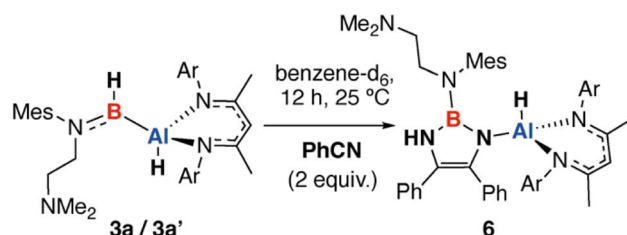
Scheme 3 Reaction of alumaborane 3a/3a' with PhCN to form a product containing a 1,3,2-diazaborole motif.
