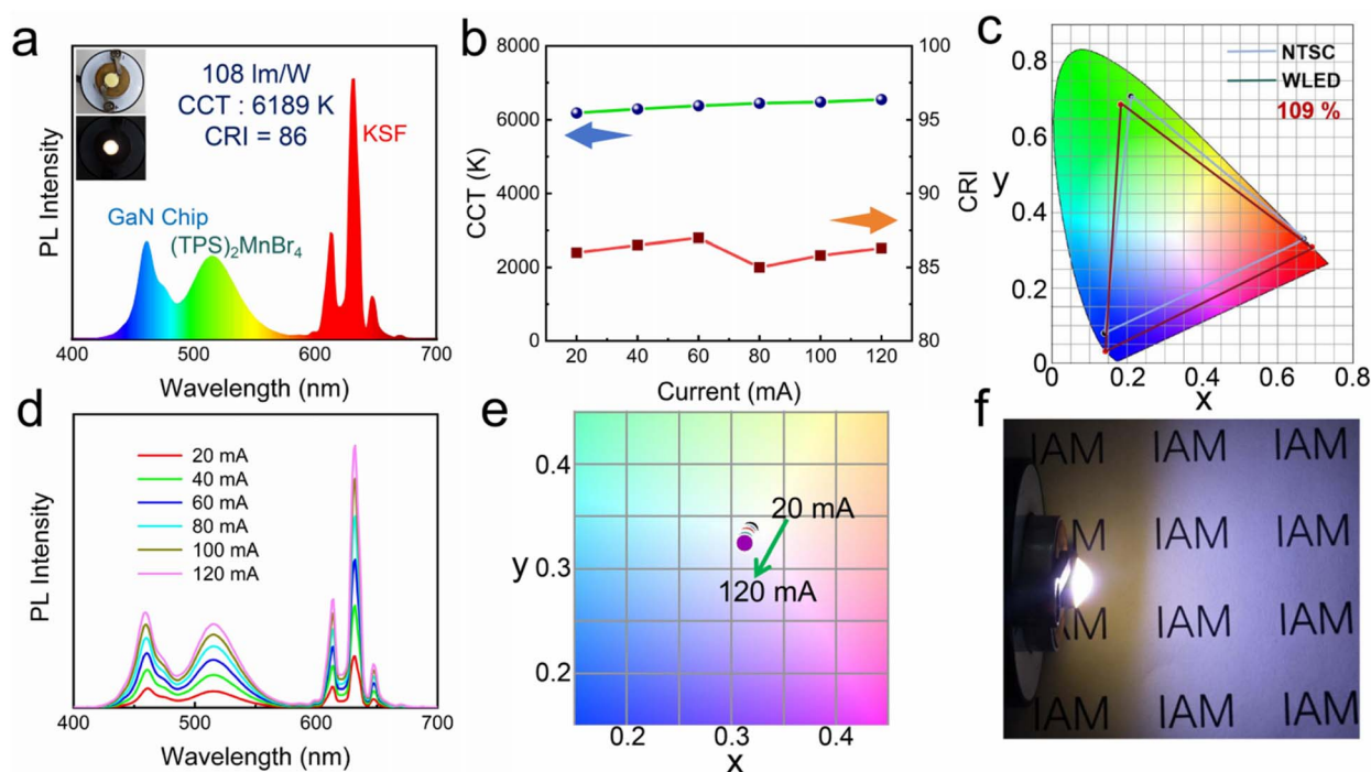
Fig. 4 (a) EL spectrum of the WLED (driven at 20 mA), composed of emission from the blue InGaN chip, green (\text{TPS})_2\text{MnBr}_4 , and red \text{K}_2\text{SiF}_6:\text{Mn}^{4+} (KSF) phosphor. Insets show photographs of the packaged device off (top) and emitting white light (bottom). (b) Variation of the CRI and CCT of the WLED as a function of driving current (20–120 mA). (c) Color gamut of the WLED and the NTSC standard in CIE 1931 chromaticity coordinates. (d) EL spectra of the WLED recorded at various driving currents (20–120 mA). (e) CIE 1931 chromaticity coordinates of the WLED plotted for different driving currents (20–120 mA). (f) Photograph demonstrating the bright white light illumination produced by the fabricated WLED device.
