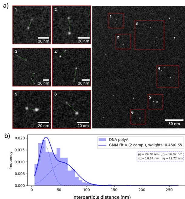
Fig. 2 (a) HAADF-STEM images of AuNP@polyA in a liquid environment, showing the presence of dimers and individual particles. (b) Two-component Gaussian mixture model (GMM) showing the presence of AuNP@polyA duplexes and single AuNP@polyA.
