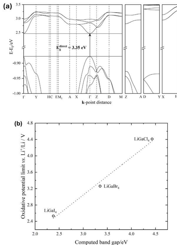
Fig. 3 (a) Computed (DFT/PBE) band structure of LiGaBr 4 with band energies scaled to the Fermi level ( E_F ). (b) Correlation between computed oxidative potential limit 12 and computed band gap energies of LiGaX 4 (X = Cl, Br, I) materials. The dotted line corresponds to a linear fit ( R^2 = 0.991 ).
