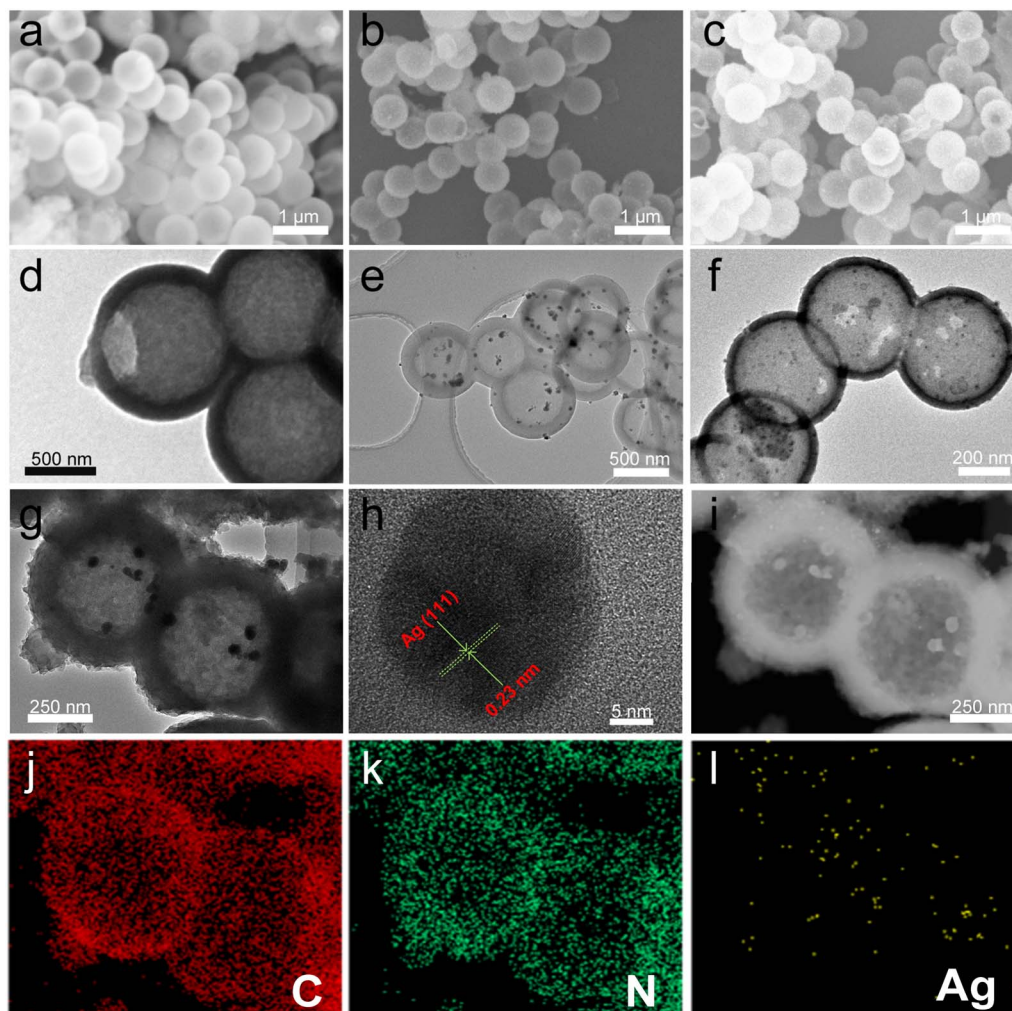
Fig. 2 SEM images of (a) SiO 2 , (b) SiO 2 @Ag@ICOFs and (c) Ag@ICOFs. TEM images of (d) SiO 2 , (e) SiO 2 @Ag and (f and g) Ag@ICOFs. (h) High-resolution TEM image displaying lattice fringes of the Ag nanoparticles. (i) Three-dimensional image. Dark-field scanning TEM image of Ag@ICOFs. (j–l) Elemental mapping images of C, N, and Ag in Ag@ICOFs.
