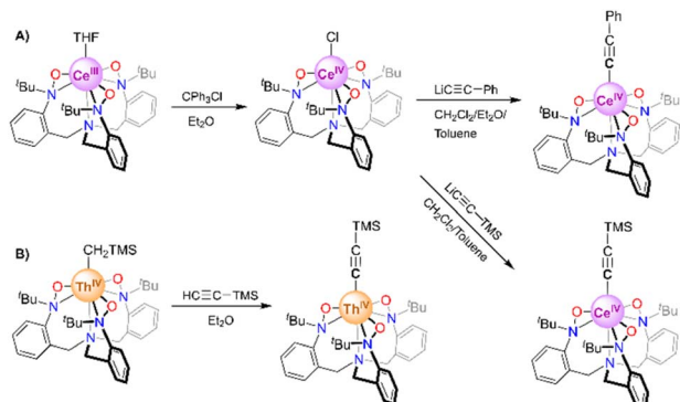
Fig. 2 Syntheses of (A) \text{Ce}^{\text{IV}} -alkynyl complexes ( 1-Ce Ph and 1-Ce TMS ) and (B) \text{Th}^{\text{IV}} -alkynyl complex ( 1-Th TMS ).
