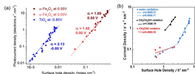
Fig. 8 (a) Rate law analyses showing the reaction order of PEC methanol oxidation on \alpha -Fe 2 O 3 at 0.55 V Ag/AgCl (dark red) and 0.00 V Ag/AgCl (light red), and on TiO 2 at -0.80 V Ag/AgCl (blue). Reproduced with permission under the terms of a CC BY 4.0 license. 99 Copyright 2017, American Chemical Society. (b) Rate law analyses showing the reaction order of PEC water oxidation at 1.3 V RHE (blue), ethanol oxidation at 1.2 V RHE (black), and acetaldehyde oxidation at 1.1 V RHE (red) on \alpha -Fe 2 O 3 . Reproduced with permission. 100 Copyright 2022, John Wiley and Sons.
