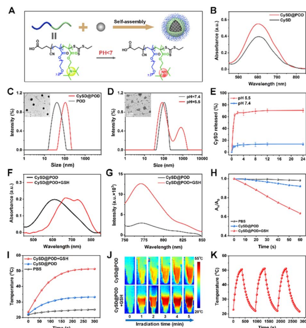
Fig. 3 (A) Schematic illustration of the pH-responsive release of CySD@POD assemblies. (B) UV-vis absorption curves of CySD and CySD@POD. Hydrodynamic size distributions and the inset shows the TEM image of CySD@POD in PBS solution at (C) pH = 7.4 and (D) pH = 5.5. (E) CySD release profiles of CySD@POD at different pH values. (F) UV-vis absorption spectra and (G) fluorescence spectra of CySD@POD before and after response to GSH. (H) Absorbance variation of DPBF at 425 nm with PBS, CySD@POD and CySD@POD + GSH under light irradiation at predetermined time points. Laser: 750 nm, 0.1 W cm -2 . (I) Photothermal heating curves of PBS, CySD@POD and CySD@POD + GSH in PBS. (J) Photothermal images of CySD@POD before and after response to GSH under light irradiation. (K) Three cycles of heating-cooling processes of CySD@POD + GSH. Laser: 750 nm, 0.5 W cm -2 .
