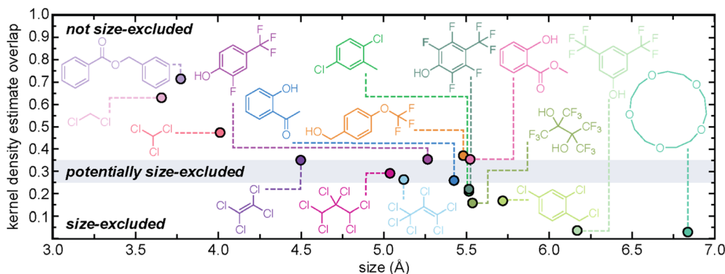
Fig. 5 Previously reported solvents whose size-exclusivity from scrambled 3^3:13^3 -R POC is known from experiment. Solvents are labelled as size-excluded (KDE overlap < 0.25), potentially size-excluded (0.25 < KDE overlap < 0.35), or not size-excluded (KDE overlap > 0.35), based on the calculated KDE overlap.
