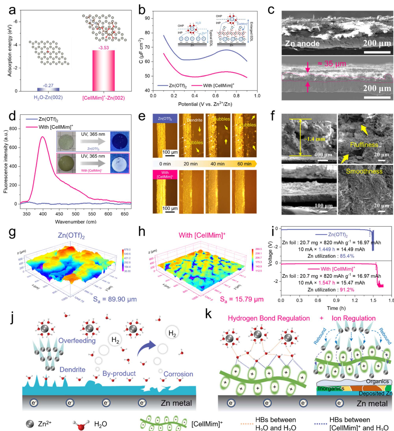
Fig. 3 (a) Adsorption energies of the Zn (002) plane with \text{H}_2\text{O} and [\text{CellMim}]^+ . (b) Differential capacitance curves of Zn||Ti half cells using \text{Zn}(\text{OTf})_2 and \text{Zn}(\text{OTf})_2 with [\text{CellMim}]^+ electrolytes. (c) Cross-section SEM images of Zn foil after immersion in different electrolytes for 10 days. (d) Fluorescence spectra of \text{Zn}(\text{OTf})_2 and \text{Zn}(\text{OTf})_2 with [\text{CellMim}]^+ electrolytes under 353 nm excitation light. The illustrations are soaked pieces of Zn foil under 365 nm UV light irradiation. (e) In situ optical microscopy images of the Zn deposition process at 10 \text{mA cm}^{-2} in different electrolytes. (f) The cross-section and surface SEM images of the Zn anode after Zn deposition for 60 min. The 3D CLSM images after Zn deposition for 60 min at 10 \text{mA cm}^{-2} in (g) \text{Zn}(\text{OTf})_2 and (h) \text{Zn}(\text{OTf})_2 with [\text{CellMim}]^+ electrolytes. (i) Cumulative plating test for Zn||Zn symmetric cells using \text{Zn}(\text{OTf})_2 and \text{Zn}(\text{OTf})_2 with [\text{CellMim}]^+ electrolytes. (j) and (k) Schematic illustration of the evolution process during Zn deposition and SEI generation in these electrolytes.
