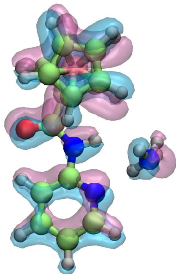
Fig. 5 Electron density difference plot comparing the neutral (red) and cationic (blue) forms of the Fcpy with ammonia, with an isovalue of 0.025, showing the redistribution of electron density upon ionization.
