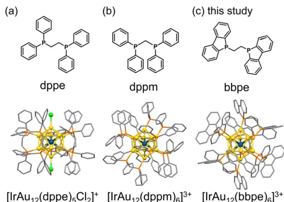
Fig. 1 The molecular structures of the diphosphine ligands and the corresponding IrAu 12 clusters for (a) [IrAu 12 (dppe) 5 Cl 2 ] + (IrAu 12 -e-Cl), (b) [IrAu 12 (dppm) 6 ] 3+ (IrAu 12 -m) and (c) [IrAu 12 (bbpe) 6 ] 3+ (IrAu 12 -b).
