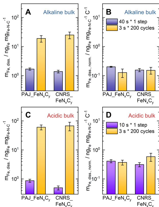
Fig. 6 The Fe dissolution data of PAJ_ \text{FeN}_x\text{C}_y and CNRS_ \text{FeN}_x\text{C}_y during the 200-cycle AST (each cycle: 3 s at j'' \text{ mA cm}^{-2} and 3 s at -0.1 \text{ mA cm}^{-2} , yellow bars) and the t -s galvanostatic step at j'' \text{ mA cm}^{-2} . The duration t of the galvanostatic step is 40 s in alkaline media (A & B, indigo bars) or 10 s in acidic media (C & D, violet bars), and the current density j'' is -75 \text{ mA cm}^{-2} for CNRS_ \text{FeN}_x\text{C}_y in Acidic-HT, and -100 \text{ mA cm}^{-2} for all the others (see Table 1). The amount of the dissolved Fe species has been normalized to the catalyst loading (A & C) or both the catalyst loading and the ORR charge (B & D). The error bars are equal to the differences between the results of the two measurements.
