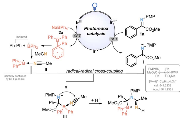
Scheme 2 Proposed mechanism.
