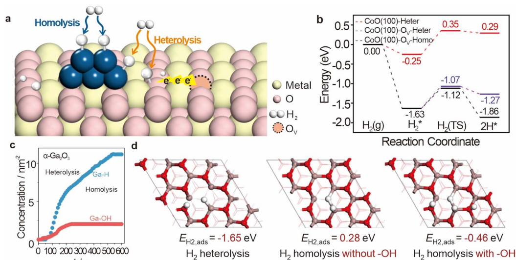
Fig. 5 (a) Mechanism of oxygen vacancies affecting hydrogen dissociation. (b) Calculated energy profiles of adsorption and dissociation of H 2 . Reproduced from ref. 30. Copyright 2022 Springer Nature. (c) The evolution of surface Ga–H and Ga–OH over α-Ga 2 O 3 samples with contact time of H 2 at 350 °C. (d) H 2 adsorption energy by homolytic dissociation over α-Ga 2 O 3 (001). Reproduced from ref. 29. Copyright 2024 Springer Nature.
