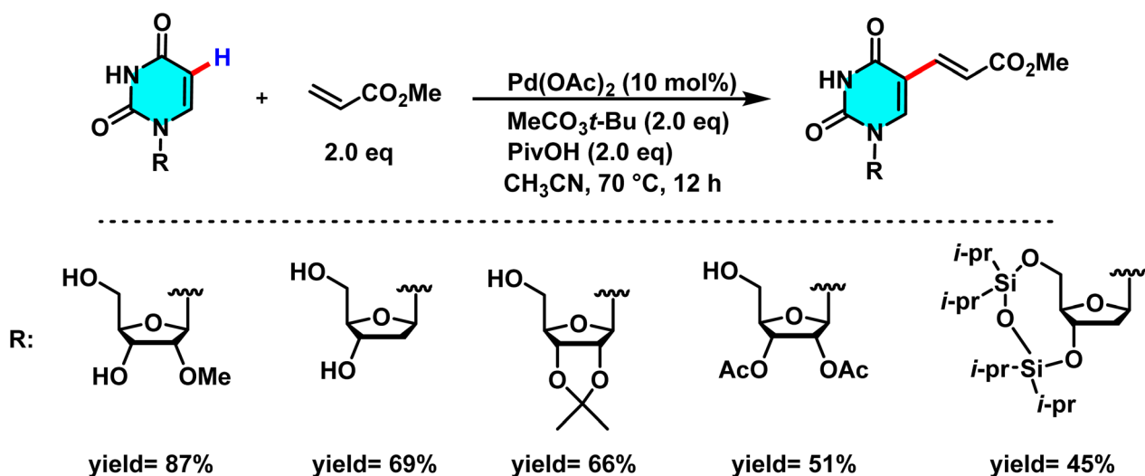
Scheme 22 C(5)-H olefination of uridine, deoxyuridine in the presence of \text{Pd}(\text{OAc})_2 .
