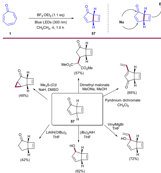
Scheme 35 Lewis acid-catalyzed 4\pi -photocyclization of tropone.
