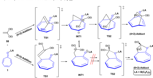
iii) Pathways for the reaction of 1 with 58 catalyzed by BPh_3
