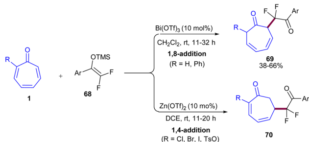
Scheme 43 Bi(OTf) 3 -promoted reaction of tropone with difluoroenoxy silanes.
