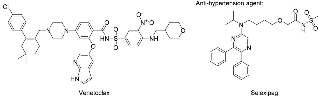
Venetoclax
