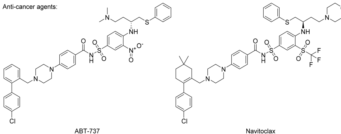
ABT-737
