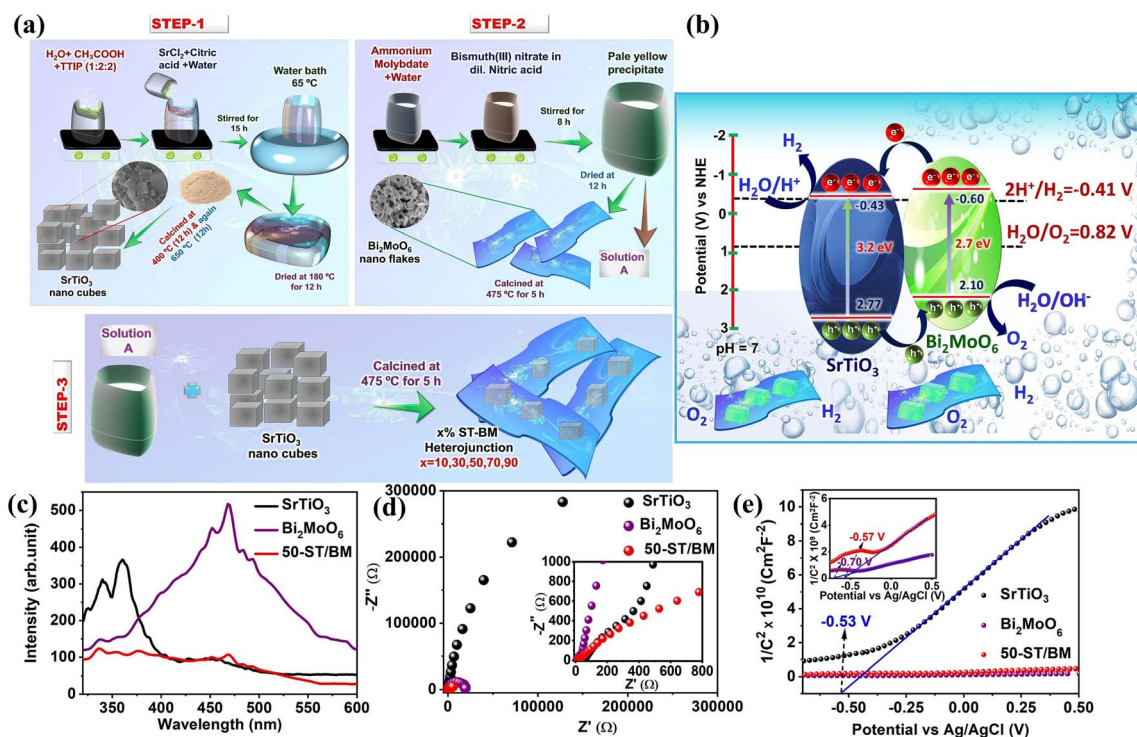
Fig. 6 (a) Overall synthesis procedure for 3D \text{SrTiO}_3 nanocubes (step 1), 2D \text{Bi}_2\text{MoO}_6 nanoflakes (step 2), and x% \text{SrTiO}_3/\text{Bi}_2\text{MoO}_6 heterojunction nanocomposite (step 3). (b) The photocatalytic overall water splitting mechanism of 50- \text{SrTiO}_3/\text{Bi}_2\text{MoO}_6 nanocomposite. (c) PL spectra (d) EIS Nyquist plots and (e) the Mott-Schottky plots of \text{SrTiO}_3 , \text{Bi}_2\text{MoO}_6 , and 50- \text{SrTiO}_3/\text{Bi}_2\text{MoO}_6 nanocomposite. Reproduced from ref. 65 with permission from Elsevier. Copyright 2025. Note: "ST/BM" in this figure denotes \text{SrTiO}_3/\text{Bi}_2\text{MoO}_6 .
