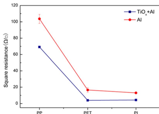
Fig. 8 Comparison of sheet resistivity for Al films with different substrates.
