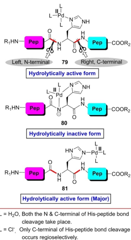
Fig. 6 Modes of co-ordination of Pd(II)-complex with histidyl peptide. Reaction conditions: (a) histidyl peptide, cis -[Pd(en)(H 2 O) 2 ] 2+ , HBF 4 (promoter), pH 1.5–2 (0.1 M HCl or 70% HCOOH), 40 °C, 2 days, 60–80%.
