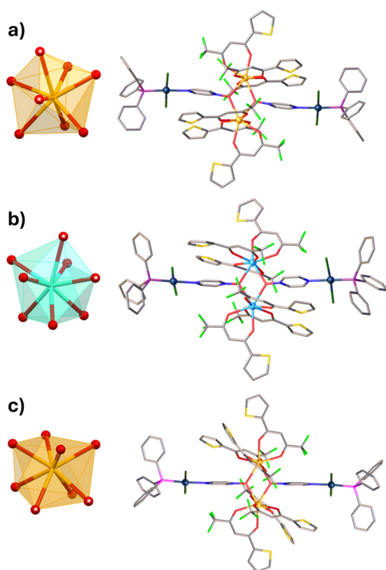
Fig. 1 Molecular structure and coordination polyhedra of the \text{LnO}_8 core for (a) 1 , (b) 2 , (c) 3 Solvent molecules, hydrogen atoms and disordered parts are omitted for clarity. Colour code: C, grey; O, red; N, blue; S, yellow; F, light green; Cl, dark green; P, violet; As, pink; Pt, dark blue; Eu, orange; Gd, azure. Oxygen atoms marked with the white asterisk belong to the bridging pyrzMO units.
