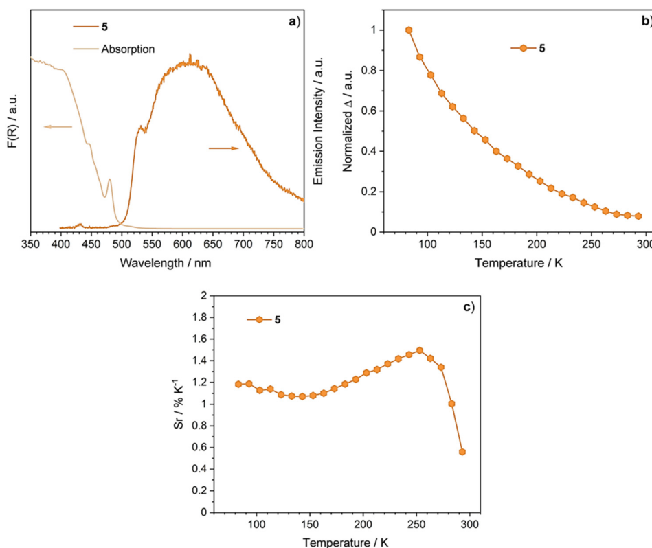
Fig. 8 Spectroscopic characterization and thermometric properties of compound 5 powders: (a) diffuse reflectance and emission spectra ( \lambda_{\text{exc}} = 400\text{ nm} ), (b) thermometric parameter \Delta defined as the integrated intensity of the emission band. (c) Relative thermal sensitivity.
