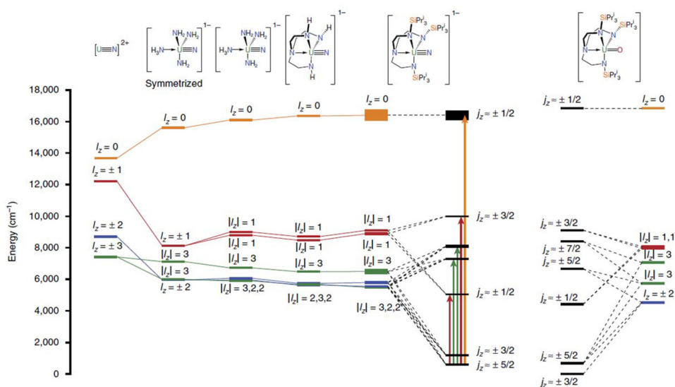
Fig. 17 The energy level splitting of five ground KDs of [U(O)(Tren^{TIPS})] ( 28 ), [U(Tren^{TIPS})(N)][M(crown)_2] ( 29 ), [U(Tren^{TIPS})(\mu-N)\{M(crown)\}] ( 30 ) and their precursors. Reprinted from the ref. 97 with permission from Springer Nature Publishing Group.
