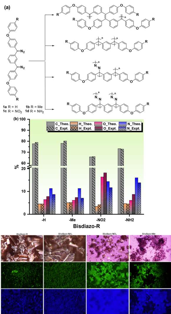
Fig. 1 (a) Chemical structures of bisdiazio-R compounds 1a–d and the possible repeating units of polymers under catalyst-free polymerization. (b) Elemental analysis and (c) optical and fluorescence images of bisdiazio-R compounds 1a–d with various terminal groups ( R = H , Me , NO_2 and NH_2 ).
