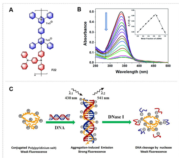
Fig. 9 (A) Structure of CMCP P22 . (B) UV-vis absorption spectra of P22 ( [\text{P22}] = 5 \mu\text{M} ) in the presence of different concentrations of ctDNA in \text{CH}_3\text{CN}-\text{H}_2\text{O} ( v/v = 1:1 ). Inset: Job's plot. A_0 is the initial absorbance of free P22 , A_1 is the recorded absorbance of complexes at different ctDNA concentrations in \text{CH}_3\text{CN}-\text{H}_2\text{O} ( v/v = 1:1 ), and X_i is the molar fraction of ctDNA. (C) Graphical abstract of the fluorescence sensing of DNA. Adapted with permission from ref. 28. Copyright 2015 the Royal Society of Chemistry.
