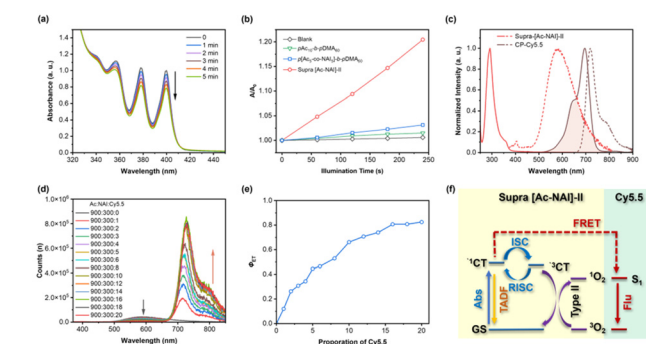
Fig. 5 (a) UV-vis absorption spectra of supra [Ac-NAI]-II/ABDA mixture under continuous irradiation (350 nm); (b) ^1\text{O}_2 generation efficiencies of supra [Ac-NAI]-II and its building units monitored by recording the absorbance of ABDA at 400 nm; (c) normalized UV-vis absorption spectra (solid curves) and fluorescence spectra (dash curves) of supra [Ac-NAI]-II and CP-Cy5.5; (d) fluorescence spectra of supra [Ac-NAI]-II co-assembled with different molar ratios of CP-Cy5.5; (e) energy transfer efficiency ( \Phi_{\text{ET}} ) at different CP-Cy5.5 molar ratios; (f) scheme of multi-channel photo-functional system based on supra [Ac-NAI]-II.
