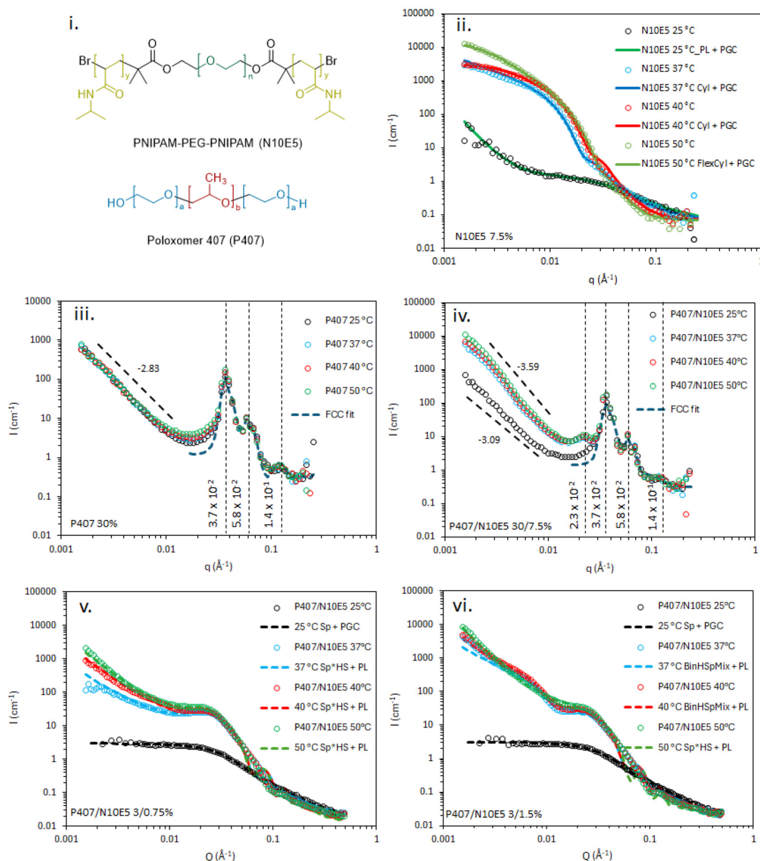
Fig. 2 (i) Chemical structure of N10E5 and P407. (ii) SANS profiles (open symbols) and fits (solid lines) of N10E5 (7.5 wt%) in D 2 O at 25, 37, 40 and 50 °C. (iii) SANS of P407 (30 wt%) at 25–50 °C with overlaid dashes highlighting peak positions. Fit to the FCC paracrystal model in mid-to-high q included as a blue dashed line. (iv) SANS of P407 (30 wt%) + N10E5 (7.5 wt%) at 25–50 °C with overlaid dashes highlighting peak positions. (v) SANS data N10E5 0.75 wt% P407 3.0 wt% and (vi) N10E5 1.5 wt% P407 3.0 wt% copolymers as a function of temperature. The abbreviations refer to the form and structure factors used: PL, power law; Sp, sphere; HSp, hard sphere; PGC, polymeric gaussian coil; Cyl: cylinder, and FlexCyl: flexible cylinder. BinHSpMix, binary mixture of spheres + hard sphere, respectively.
