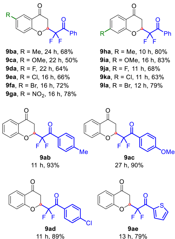
Fig. 3 Highly efficient Michael addition of difluoroenoxyisilane 8a – e to chromones 1a – e .
