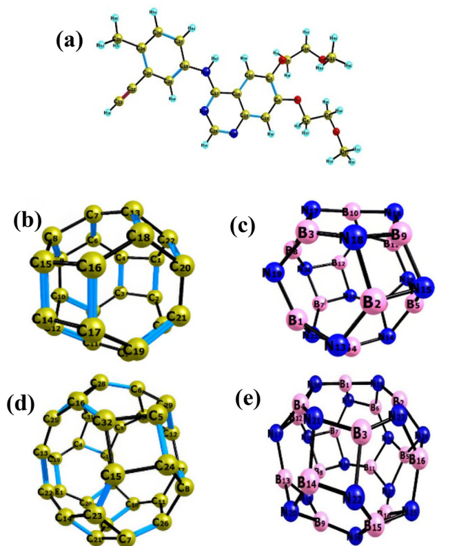
Fig. 1 Optimized structures of (a) the methyl erlotinib molecule, (b) C_{24} nanocage, (c) B_{12}N_{12} nanocage, (d) C_{32} nanocage and (e) B_{16}N_{16} nanocage.
