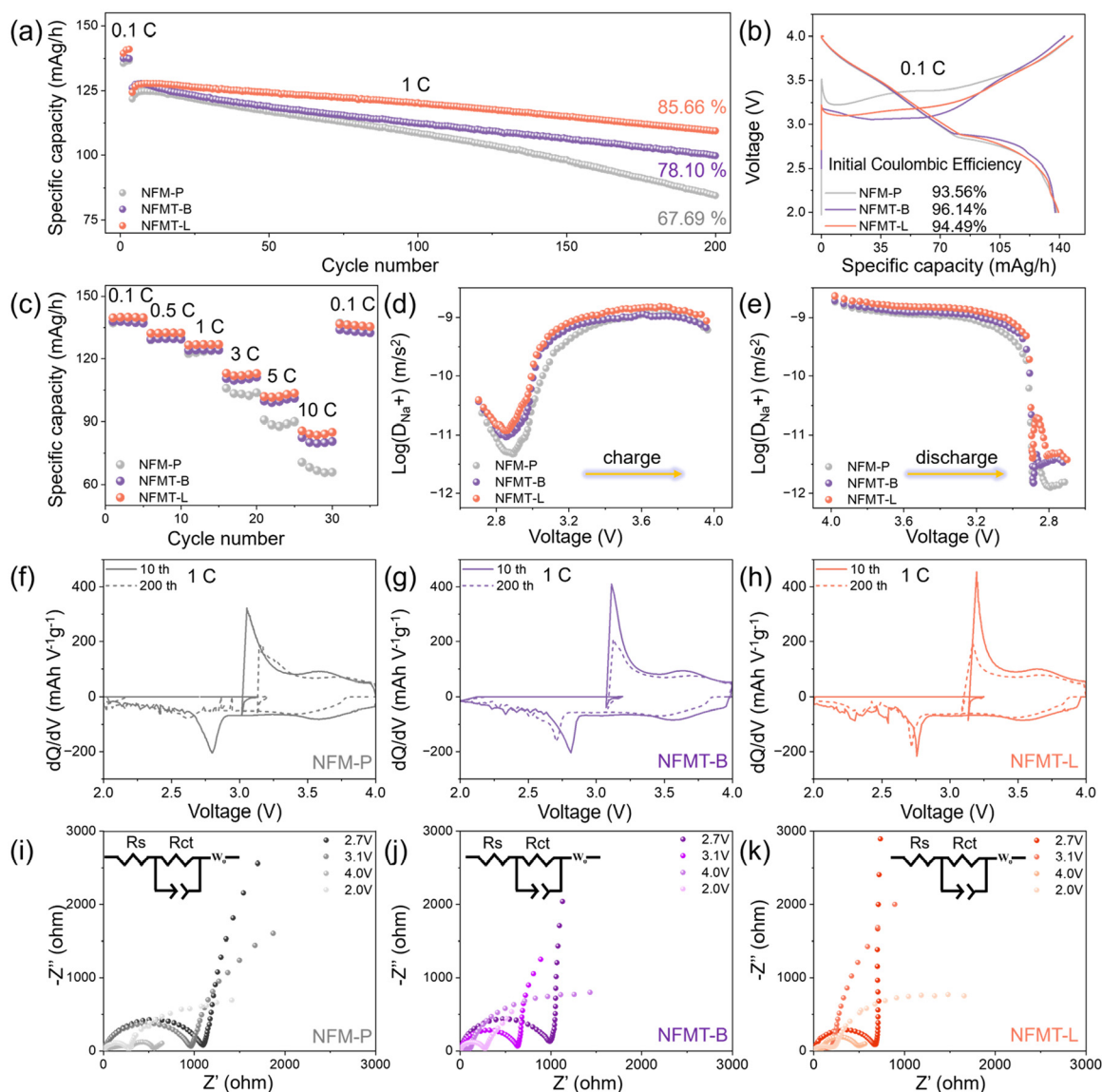
Fig. 6 (a) Cycling performance; (b) the first charge/discharge curve at 12 \text{ mA h g}^{-1} ; (c) rate performance; (d and e) GITT-calculated diffusion coefficients ( D_{\text{Na}^+} ) of NFM-P, NFMT-B and NFMT-L; (f–h) dQ/dV curves after the 10th and 200th cycles; and (i–k) in situ EIS Nyquist plots at different potentials of NFM-P/NFMT-B/NFMT-L.
