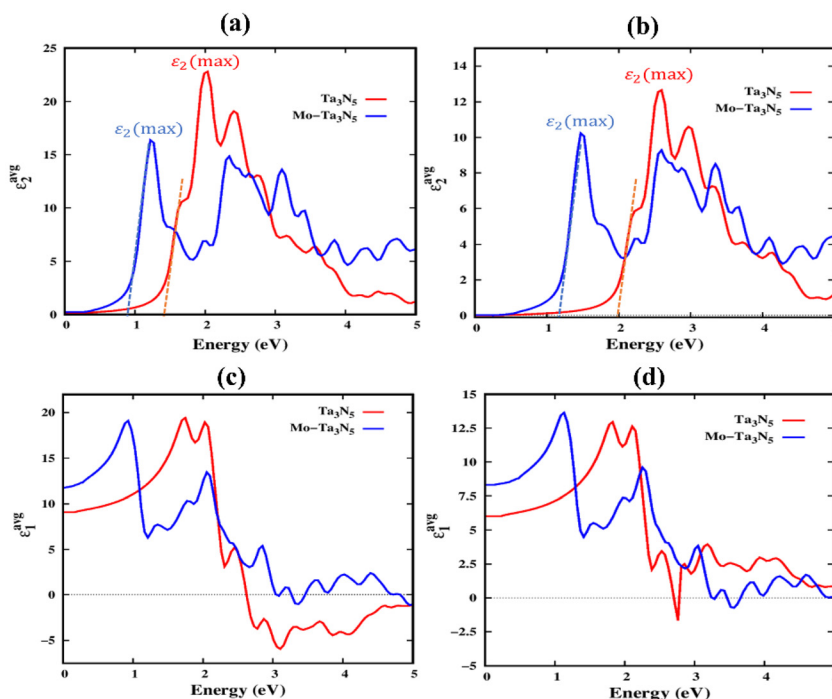
Fig. 3 (a) The imaginary part of the dielectric function for bare and Mo-doped \text{Ta}_3\text{N}_5 , calculated using GGA. (b) The imaginary part of the dielectric function for bare and Mo-doped \text{Ta}_3\text{N}_5 , obtained from GGA+U calculations. (c) The real part of the dielectric function for bare and Mo-doped \text{Ta}_3\text{N}_5 , computed using GGA. (d) The real part of the dielectric function for bare and Mo-doped \text{Ta}_3\text{N}_5 , calculated with GGA+U ( u = 0.2 ).
