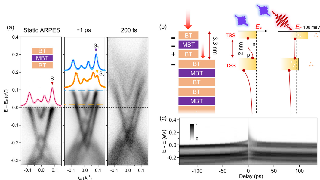
Fig. 3 Multiple surface photovoltages on the 1-BT termination. (a) Static ARPES spectrum and trARPES spectra on the 1-BT termination with momentum distribution curves (MDCs) taken at the equilibrium Fermi level (static ARPES) and the shifted Fermi levels of two replica bands at -1 ps. Peak S at equilibrium is split into peaks S_1 and S_2 at -1 ps. The time-dependent spectra were obtained using an IR pump fluence of 95 \mu\text{J cm}^{-2} . (b) Proposed charge redistribution in \text{Mn}(\text{Bi}_{0.82}\text{Sb}_{0.18})_6\text{Te}_{10} and band bending toward the surface. The cartoons illustrate the dual-SPV effect at 2 adjacent exposed 1-BT terminations. The red solid line represents the overall band bending. The black dashed line stands for the equilibrium Fermi level. (c) Time-dependent EDCs around the \Gamma point clearly show the band splitting starting from around -30 ps and lasting more than 100 ps after time zero.
