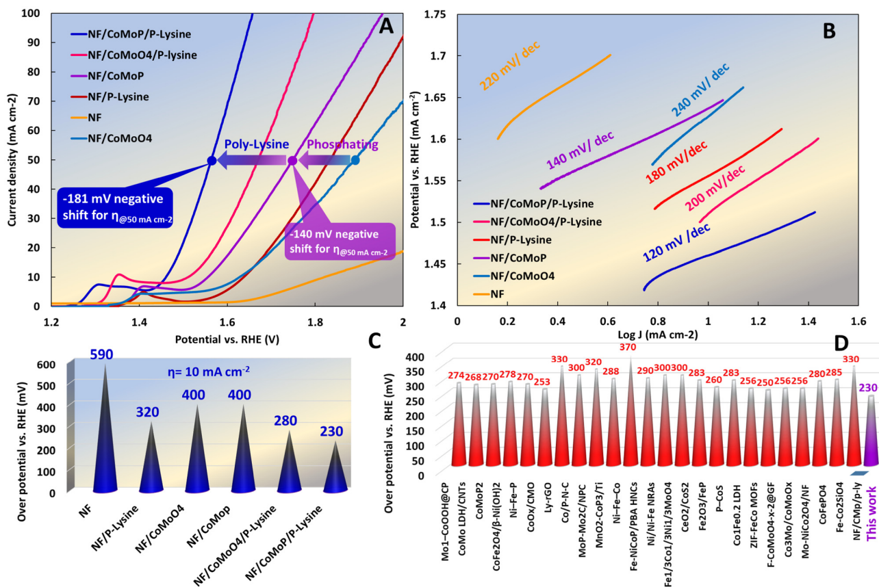
Fig. 3 Electrochemical evaluation of the OER on the as-prepared electrodes. (A) Steady-state LSV measurements at a scan rate of 5 \text{ mV s}^{-1} in 1 \text{ M KOH} and (B) the equivalent Tafel plot derived from the LSV, despite boosting the OER, NF/CoMoP/p-Lys shows the Tafel slope pushing to a theoretical value of 118 \text{ mV dec}^{-1} in the low overpotential region and seems that the first ET controls PCET as the RDS. Comparison of the required overpotentials of the (C) as-prepared electrodes together at J = 10 \text{ mA cm}^{-2} . (D) Comparison of the required overpotentials of the NF/CoMoP/p-Lys electrode with the recently published OER electrocatalysts to reach J = 10 \text{ mA cm}^{-2} (references are respectively from left to right). 35–58
