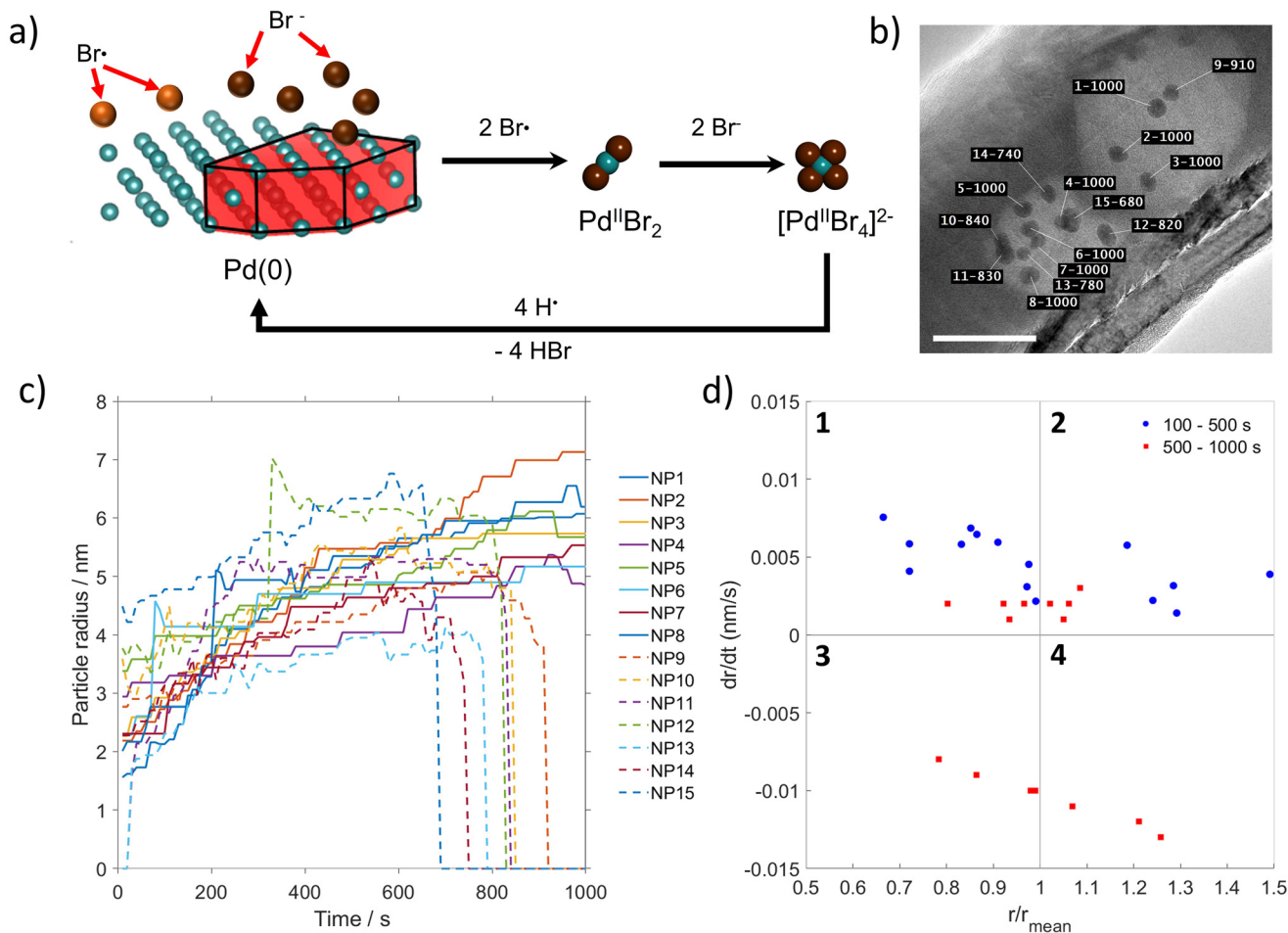
Fig. 6 (a) Oxidation of Pd(0) to Pd(II) by bromine atoms leads to full or partial dissolution of nanoparticles. [PdBr 4 ] 2- is a soluble form of Pd(II), which can be recycled to grow the next generation of nanoparticles. Reduction of Pd(II) to Pd(0) by hydrogen radicals leads to nanoparticle growth with bromide anions adsorbed on the crystal facets, thus controlling the nanoparticle shape. (b) TEM image highlighting the 15 nanoparticles in IL solution in nanotube present after 500 s of 200 keV electron beam irradiation, the numbers n – m indicate ‘number of nanoparticle’ – ‘time at which the particle was last observed’ (a value of m = 1000 indicates that the particle did not undergo dissolution within the 1000 s timeframe). (c) A graph of particle radius plotted against time shows that the Pd NP generally grew at a similar rate for the first 500 s (driven by the reduction of Pd(II) to Pd(0) through DKO) after which some particles dissolved very suddenly (dashed lines; driven by Pd(0) to Pd(II) oxidation by Br • radicals through DVE), and others experienced decreased growth. (d) The rate of growth against the normalised particle size, r/r_{\text{mean}} , allows for the trends to be observed, indicating that the change in particle size was more likely to be due to monomeric addition or migration and coalescence (a minority of cases) over Ostwald ripening. Scale bar is 50 nm.
