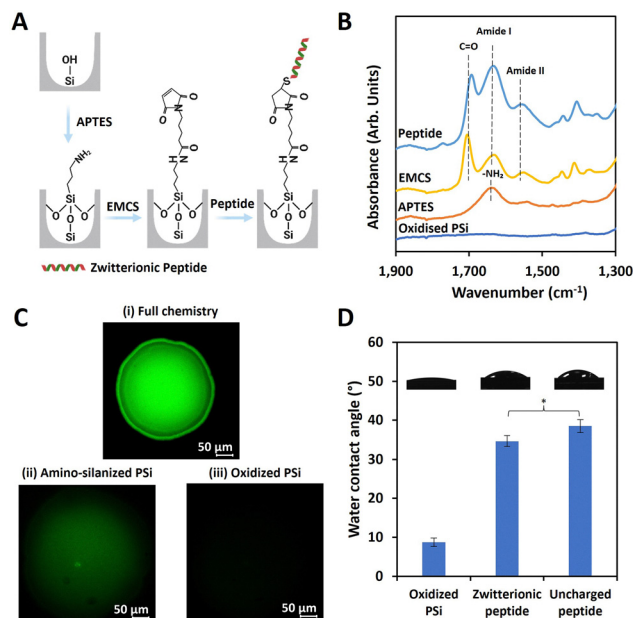
Fig. 1 Characterization of peptide conjugation on the PSi surface. (A) Schematic illustration of zwitterionic peptide immobilization onto the PSi surface. Created with https://BioRender.com . (B) ATR-FTIR spectra. (C) CLSM projection images of the PSi film conjugated with a FAM6-labeled peptide in the following cases: (i) full conjugation chemistry, (ii) control experiment with no activation of the silanized surface with the coupling agent EMCS and (iii) bare oxidized PSi. Data represented as means \pm SD, n = 3 . (D) The static water contact angle measurement on the different modified surfaces; oxidized PSi, zwitterionic peptides and uncharged peptides modified surfaces.
