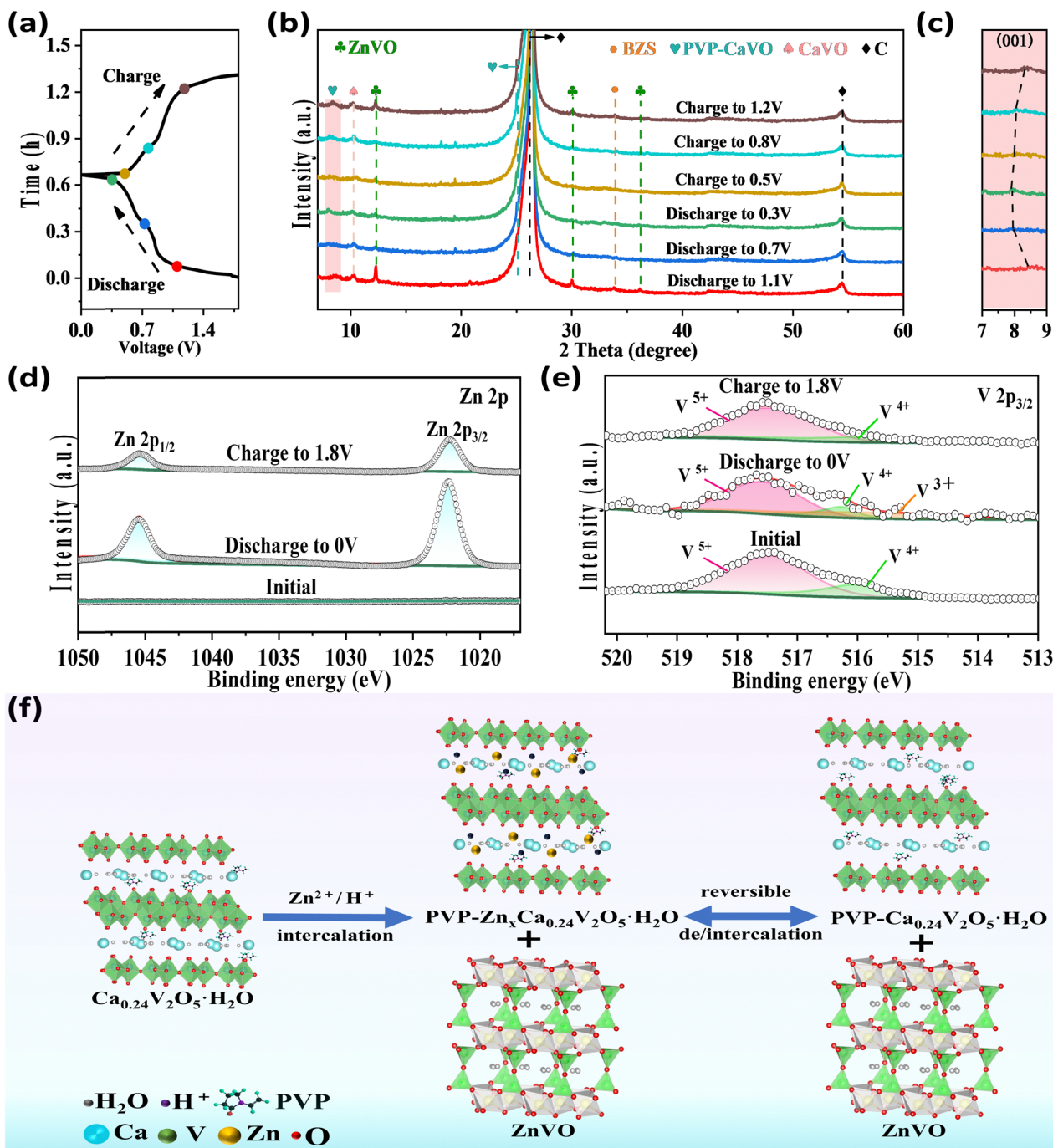
Fig. 6 (a) Discharge/charge curves of PVP-CaVO in AZIBs. (b) Ex situ XRD patterns. (c) Enlargements of patterns. (d) XPS spectra of Zn 2p. (e) XPS spectra of V 2p. (f) Schematic illustration of the \text{Zn}^{2+} storage mechanism of PVP-CaVO.
