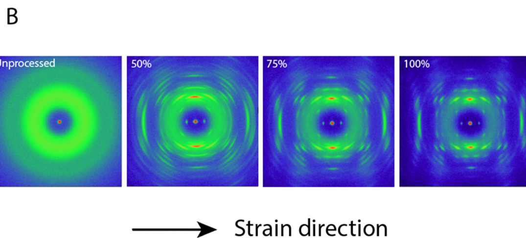
Fig. 5 (A) 1D XRD patterns of PLLA films subjected to various strain levels. Inset shows an enlarged image of the \beta -phases. (B) two-dimensional WAXS analysis illustrating changes in polymer chain orientation resulting from post-processing with the strain direction.
