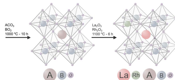
Fig. 1 Overall synthesis scheme for ABO_3 perovskites and subsequent La,Rh co-doping.
