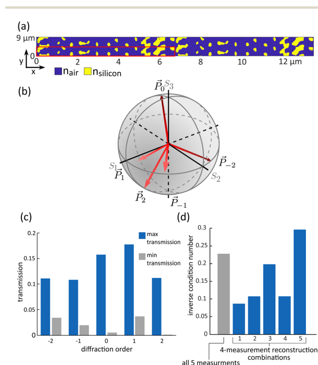
Fig. 3 (a) Optimised metasurface design for polarisation imaging for 1 \mu\text{m} thick patterned silicon on a 460 \mu\text{m} sapphire substrate. A single period is 6750 nm by 450 nm, indicated in red, and repeated across the whole metasurface. (b) The partial polarisers associated with each diffracted measurement can be plotted on a sphere, where the direction indicates the polarisation of the polariser analogous to Stokes vectors, and the magnitude of the vectors indicates the effectiveness of the polariser (c) Transmission of the ideal polarisation state and the orthogonal state for each diffraction order gives the maximum and minimum transmission possible for the order. The contrast between the maximum and minimum transmission indicates the polarisation sensitivity of the diffraction orders. (d) The inverse condition number is one measure of how robustly the polarisation measurements span the Stokes space. The inverse condition number of all possible reconstructions shows individual reconstructions sufficiently span the space for polarisation reconstruction.
