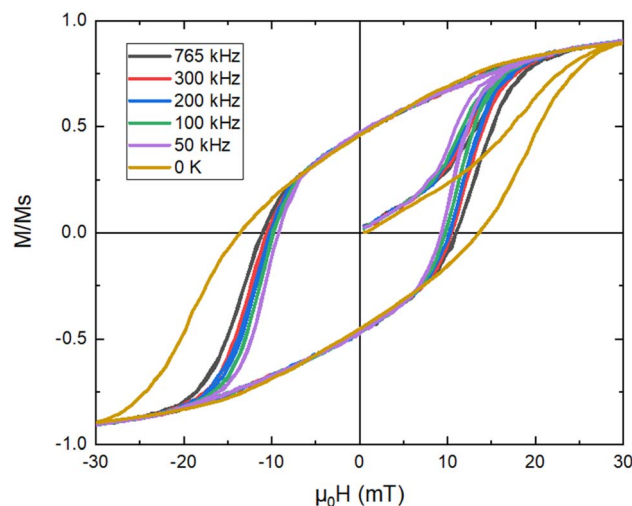
Fig. 8 AC hysteresis loops for 30 mT magnetic field amplitude and for various frequencies (50–765 kHz). The largest loop corresponds to 0 K and is independent of the frequency. 35
