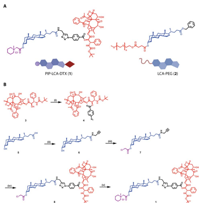
Fig. 1 (A) Chemical structures of PIP-LCA-DTX and LCA-PEG. (B) Synthetic route for the synthesis of PIP-LCA-DTX.
