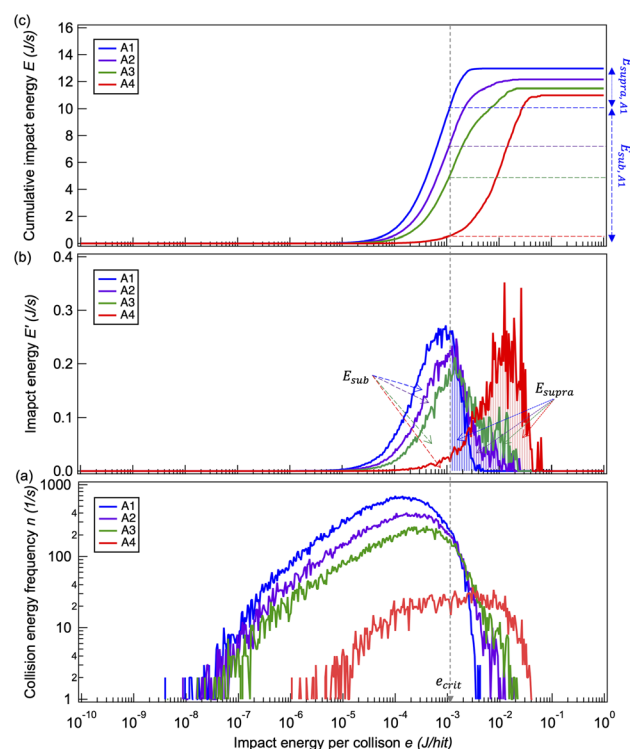
Fig. 2 (a) Distribution of collision frequency n that occurred at a certain impact energy value e under various conditions of A1, A2, A3, and A4. ( e_{\text{crit}} = 1.1 \times 10^{-3} J per hit). (b) Impact energy E' imparted to the system by collisions within a certain impact energy value e . The integrated area to the left of e_{\text{crit}} represents E_{\text{sub}} and the integrated area to the right of e_{\text{crit}} represents E_{\text{supra}} . (c) Cumulative impact energy E .
