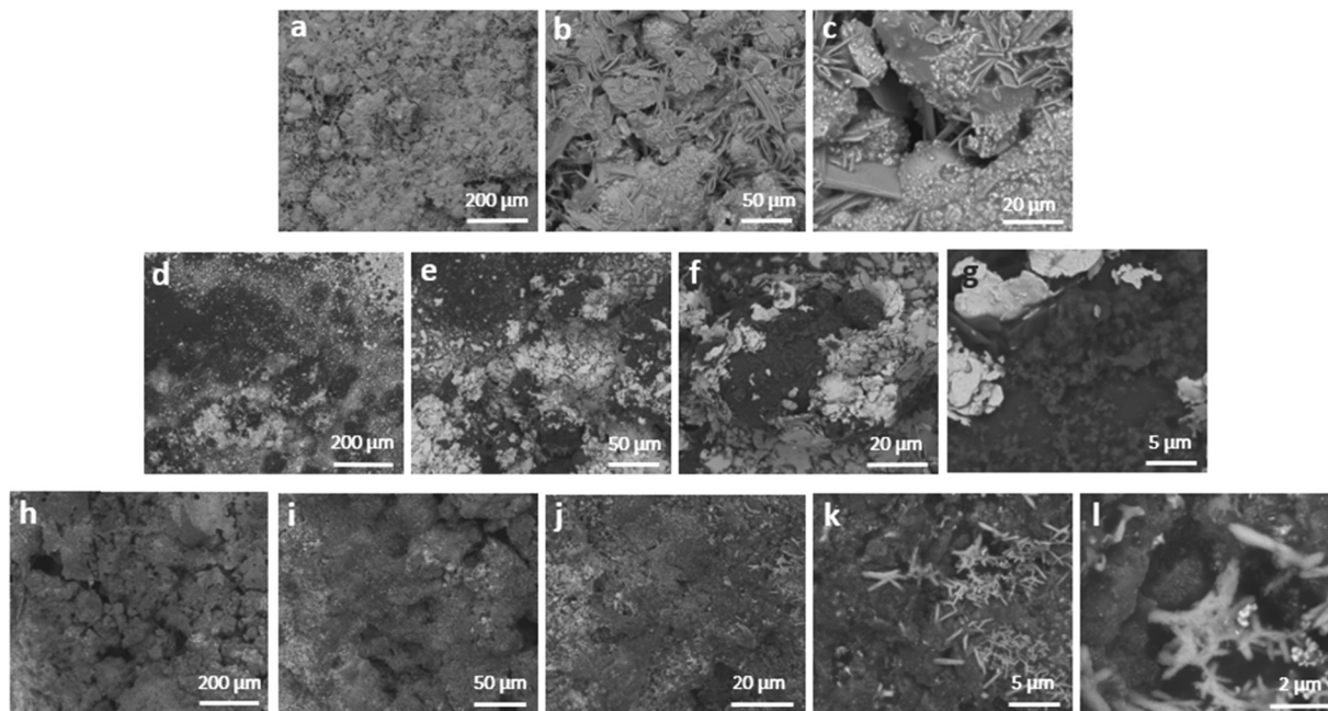
Fig. 6 (a)–(c) SEM images of IL-functionalized geopolymer samples without silver adhesive to show the natural interaction between the geopolymer and \text{EMIM}^+ \text{Otf}^- ; (d)–(g) SEM images of IL-functionalized geopolymer samples including a layer of silver adhesive on them before testing; and (h)–(l) SEM images of IL-functionalized geopolymer samples after testing. ( \phi = 1000 \mu\text{m} and h = 140 \mu\text{m} for all the samples).
