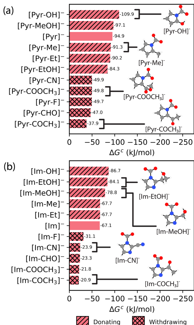
Fig. 5 The [\text{HBAA}]^- \text{CO}_2 complexation free energies (in \text{kJ mol}^{-1} ), where \Delta G^c = \Delta G_2 for the (a) [\text{Pyr}-X]^- and (b) [\text{Im}-X]^- families with different functional groups (as shown in Fig. 2). The single hatch indicates electron-donating groups and the double hatch indicates electron-withdrawing groups. The naming conventions for structures appearing in Fig. 4 are modified according to the naming convention in Fig. 2 ( i.e. , [\text{Pyr}-\text{CN}]^- = [\text{2-CNpyr}]^- , [\text{Im}-\text{Me}]^- = [\text{Melm}]^- , and [\text{Im}-\text{Et}]^- = [\text{Etlm}]^- ). Atom color key: gray = carbon, blue = nitrogen, red = oxygen, white = hydrogen.
