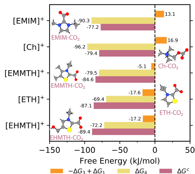
Fig. 6 The HBAC pathway free energies ( \Delta G^c = -\Delta G_3 + \Delta G_1 + \Delta G_4 ; mauve), the proton transfer free energies ( -\Delta G_3 + \Delta G_1 ; orange), and the \text{CO}_2 binding free energies ( \Delta G_4 ; yellow). \Delta G_1 is calculated using [\text{Im}]^- as the proton acceptor. The structure insets illustrate the \text{CO}_2 complexation final products. Atom color key: gray = carbon, blue = nitrogen, red = oxygen, white = hydrogen, yellow = sulfur.
