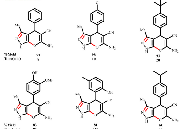
Scheme 30 Synthesis of pyrano[2,3- c ]pyrazoles using a copper-based nanocatalyst (Ali et al. ).
